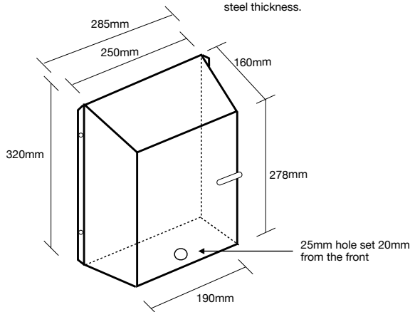
Standard Tap Box.
